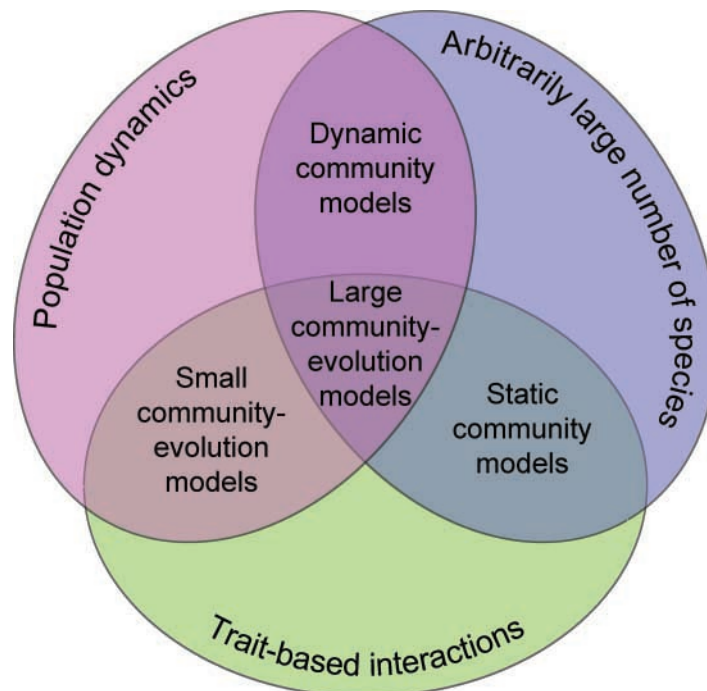
Fig. 1. Schematic illustration of the community models considered in this review. We begin by surveying static and dynamic ecological models, which do not possess an evolutionary component. Next, we move on to evolution in small community-evolution models. Finally, we review large community-evolution models (LCEMs), which synthesize elements of all aforementioned model types.
