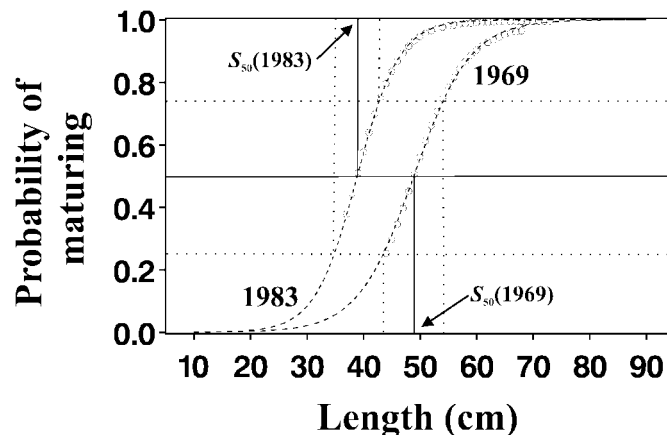
Fig. 3. Application of the estimation method for Georges Bank cod stock. Probability of maturing at age 3 computed as a function of size for cohorts 1969 and 1983. ○, raw estimations of the probabilities of maturing computed in the observed size range; —, fitted logistic regression curves. Thin solid lines (dotted) indicate how the reaction norm midpoints (quartiles) can be graphically determined.
